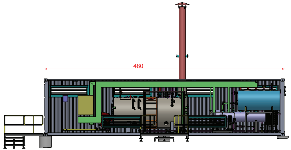
ELEVATION VIEW
