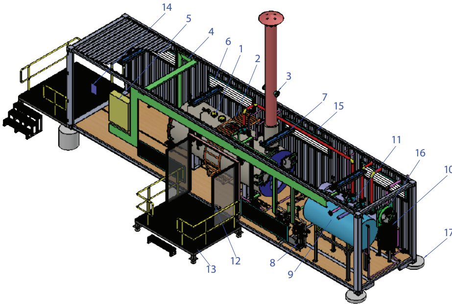
REAR VIEW
